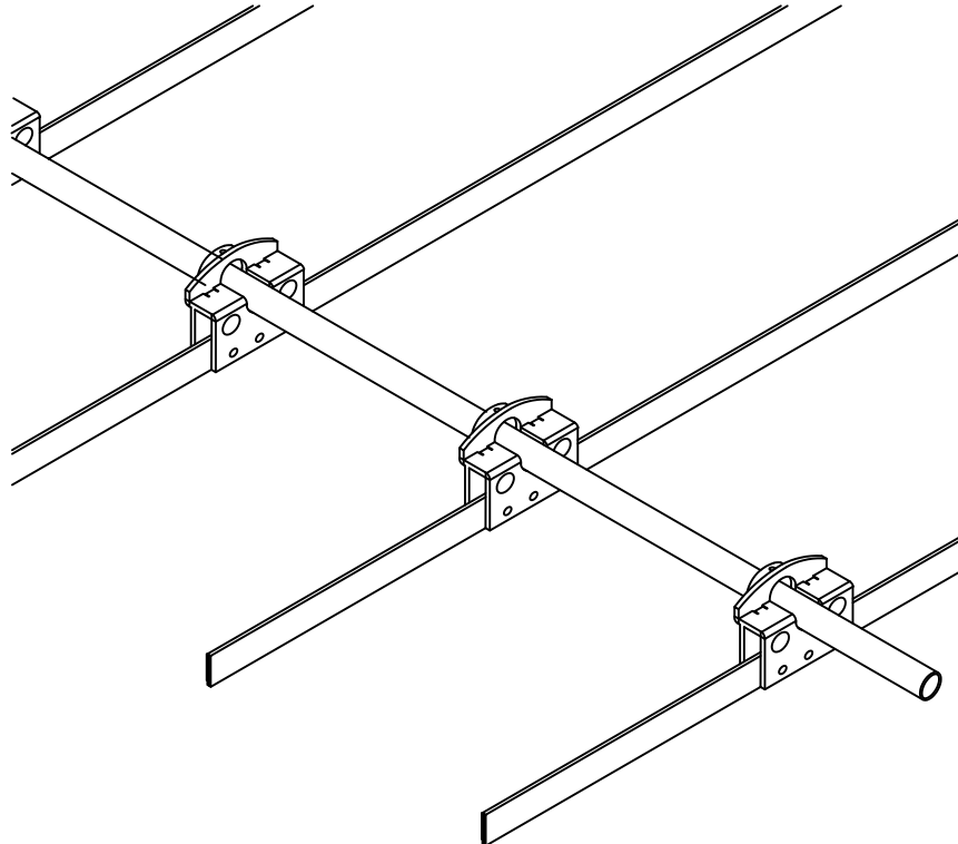
ISOMETRIC VIEW
